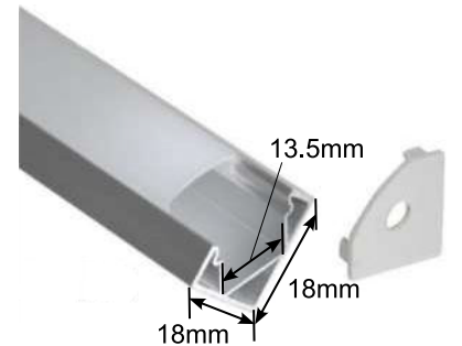
45° Corner Track AC-AL18
