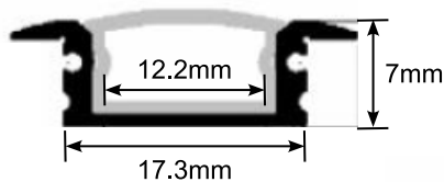
Recessed Winged Track Specifications
