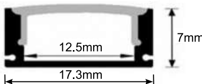
Standard Track
