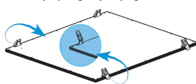
Install Spring Clips onto Panel Flip Spring Clips Upright
